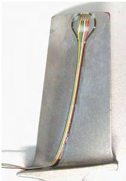
Fig. 1: Instrumented turbine blade with strain gauges.
